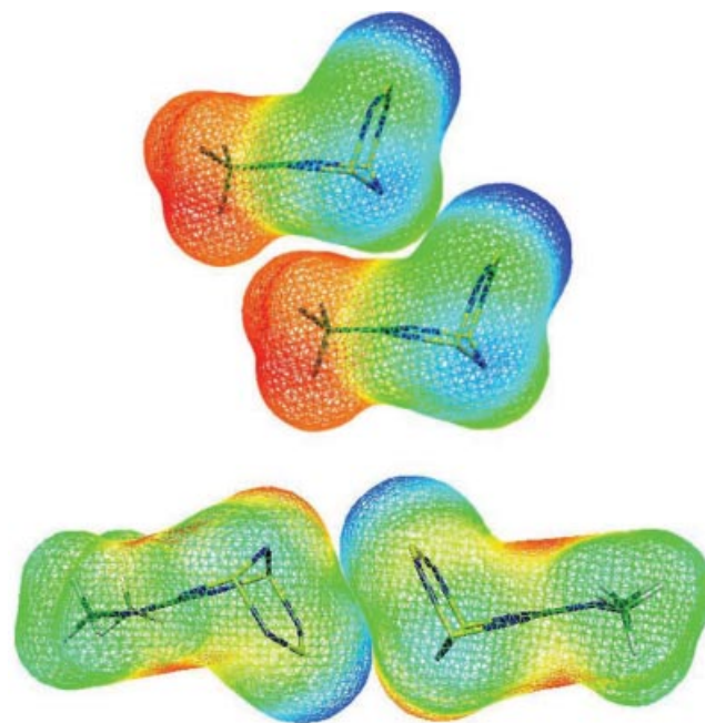
Figure 8. MEP (mapped electrostatic potential) of representative examples for stacking (R = CF 3 ) and for dimerisation (R = NMe 2 )
